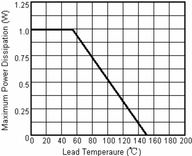
Fig.8 Power Temperature Derating Curve
